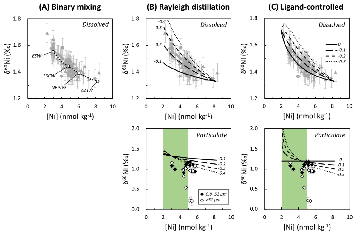
Fig. 6. Comparison of dissolved and particulate Ni isotopic composition ( d\delta^{60}\text{Ni} and p\delta^{60}\text{Ni} ) versus Ni concentrations ( d[\text{Ni}] and p[\text{Ni}] ) of samples collected in this study. Isotope systematics can be modeled as simple physical mixing between water masses, where open circles represent the d[\text{Ni}] and d\delta^{60}\text{Ni} at the depths where ESW, 13CW, NEPIW and AAIW values converge, and dashed lines between the open circles are derived from a conservative binary mixing model (A). Alternatively, the data can be modeled by Rayleigh distillation, with the data suggesting an instantaneous isotope effect ( \Delta^{60}\text{Ni}_{\text{particulate-aqueous}} ) of -0.1 to -0.4\text{‰} (B). Finally, the data can be fit by a Rayleigh fractionation model which assumes 2 nM of non-bioavailable Ni with a \delta^{60}\text{Ni} value of +1.7‰, and isotope effects from 0 to -0.3\text{‰} (C). In all plots, the gray symbols show observations from this study. For both Rayleigh models, we show the predicted instantaneous \delta^{60}\text{Ni} of phytoplankton export, compared to observed particle \delta^{60}\text{Ni} in the 0.8–51 \mu\text{m} (filled diamonds) and >51 \mu\text{m} (open diamonds) ranges, respectively. Green shaded areas show the concentration range of dissolved [\text{Ni}] in the euphotic zone (top 100 m). A value from a >51 \mu\text{m} particle sample at 25 m was identified an outlier, and is therefore not included here.
