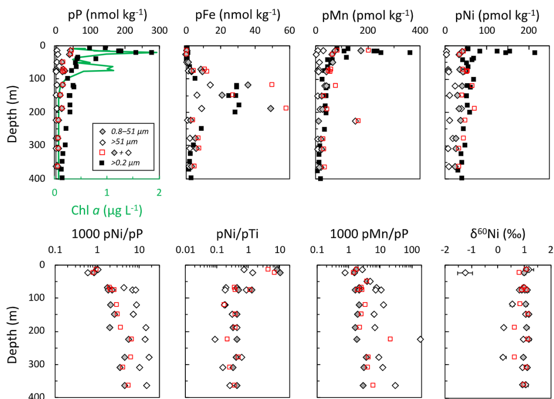
Fig. 5. Concentrations of particulate P (pP), Fe (pFe), Mn (pMn), Ni (pNi), Ni isotopic composition ( \delta^{60}\text{Ni} ), elemental ratios (including pNi/pP multiplied by 1000, pNi/pTi, and pMn/pP multiplied by 1000), and concentrations of chlorophyll a (Chl a ) throughout the water column at station P1 in 2018. Filled squares represent total suspended particles ( >0.2\ \mu\text{m} ) collected by onboard filtering of seawater. Open and gray diamonds stand for particles with sizes of 0.8\text{--}51\ \mu\text{m} and >51\ \mu\text{m} , respectively, collected from submerged McLane pumps. Red open squares represent the sum of the two McLane pump size fractions ( >0.8\ \mu\text{m} ). (For interpretation of the references to color in this figure legend, the reader is referred to the web version of this article.)
